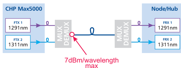
Diagram 1. 1291 and 1311 nm CWDM forward path implementation
