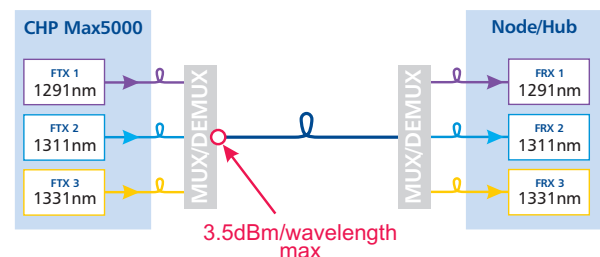
Diagram 2. 1291, 1311, and 1331 nm CWDM forward path implementation
