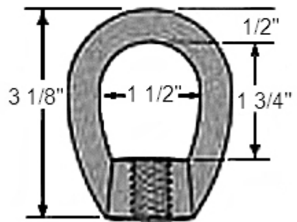
THIMBLE EYENUT FIG. 3
